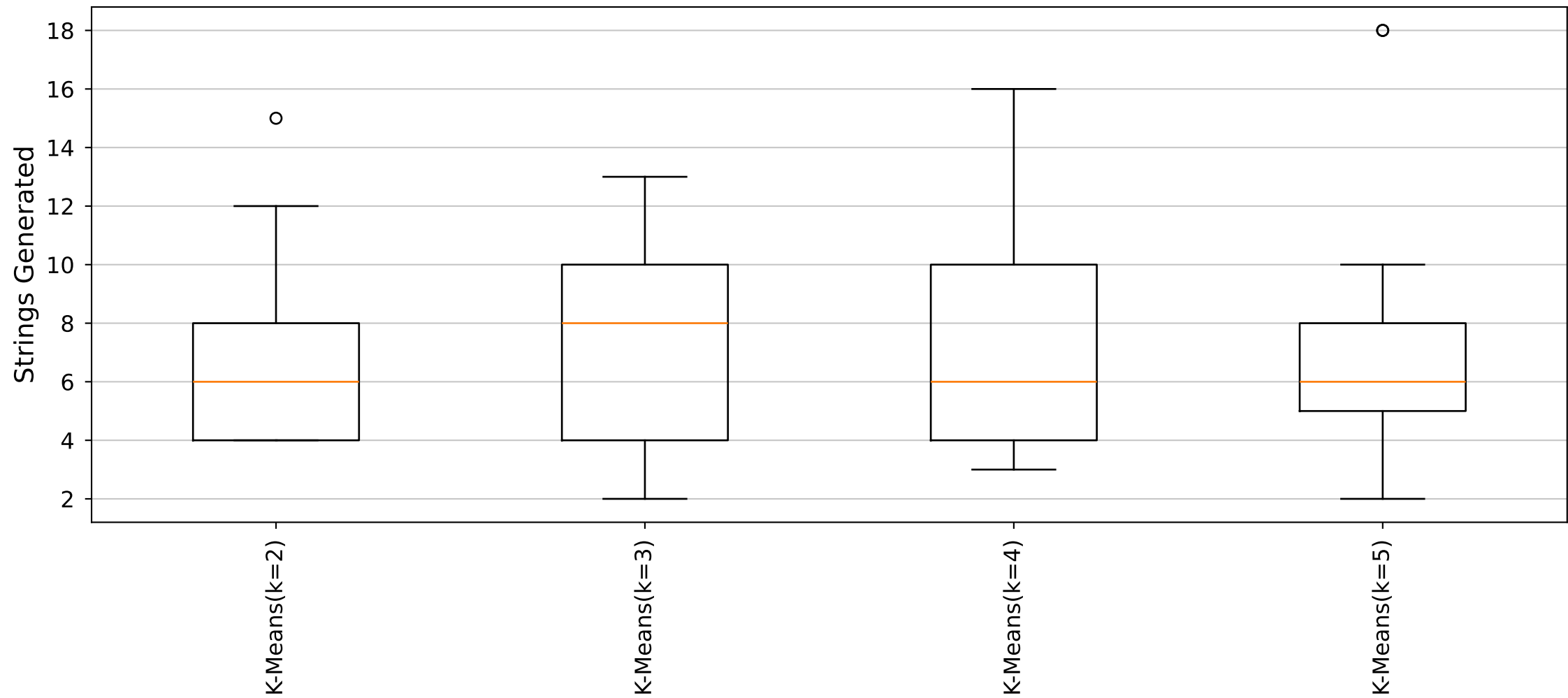
YARA Rules Strings Generated Distribution (Cluster37_Size5 dataset)
